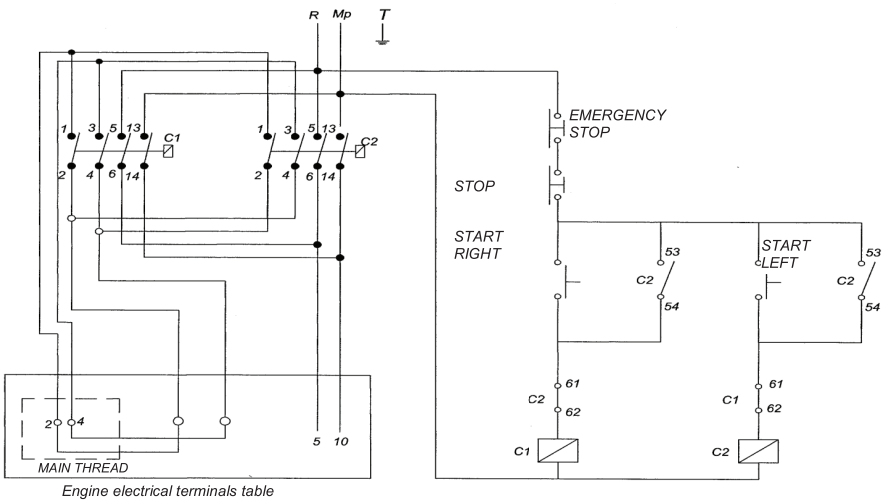
ELECTRICAL DIAGRAM FOR MONO PHASE MINCING MACHINES
