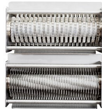
KT-PK-2 Double Tenderizer Knives
